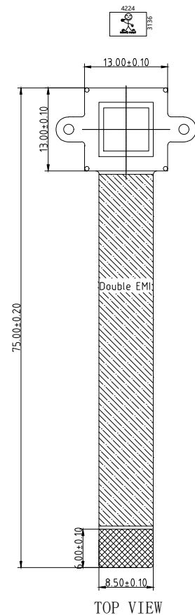
TOP VIEW
